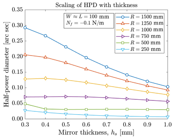
Fig. 6 HPD as a function of substrate thickness, for various radii.
